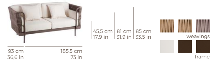
SOFÁ 2 / SOFA REF.: 77147
