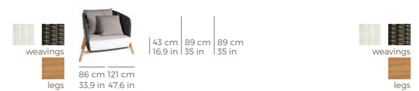
ROUND SILLÓN / ARMCHAIR REF.: 76545
